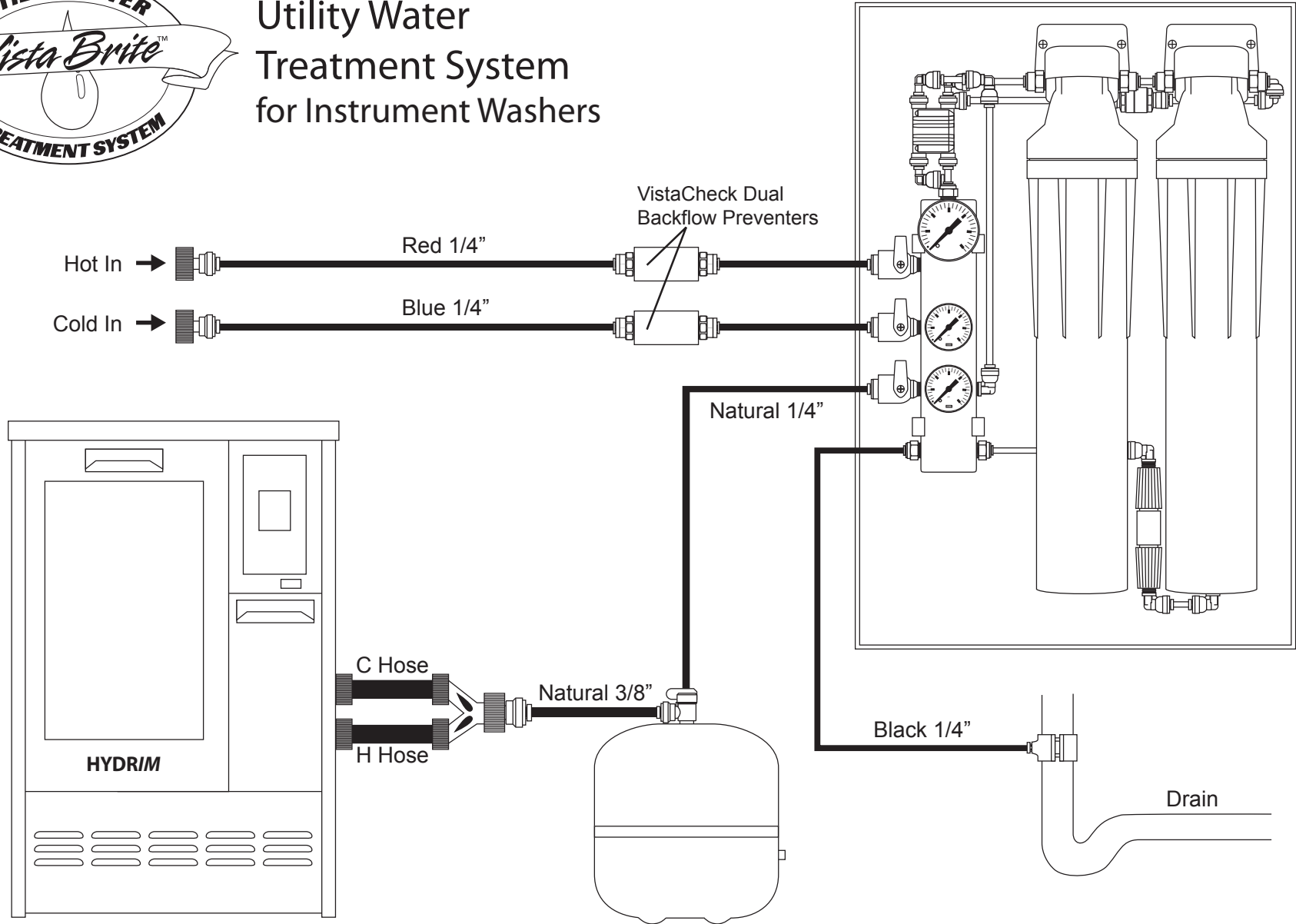
Typical Installation A For Optimal Inlet Water Pressure (50-80 psi / 3.4-5.5 bar)
