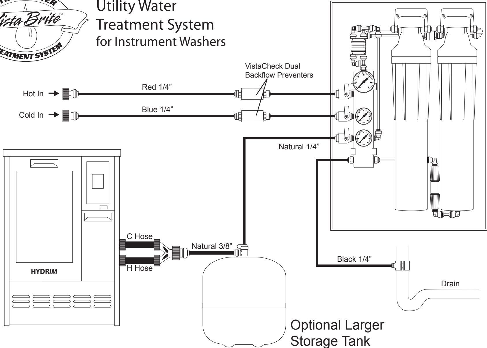
Typical Installation C For Low Inlet Water Pressure (40-50 psi / 2.8-3.4 bar)
