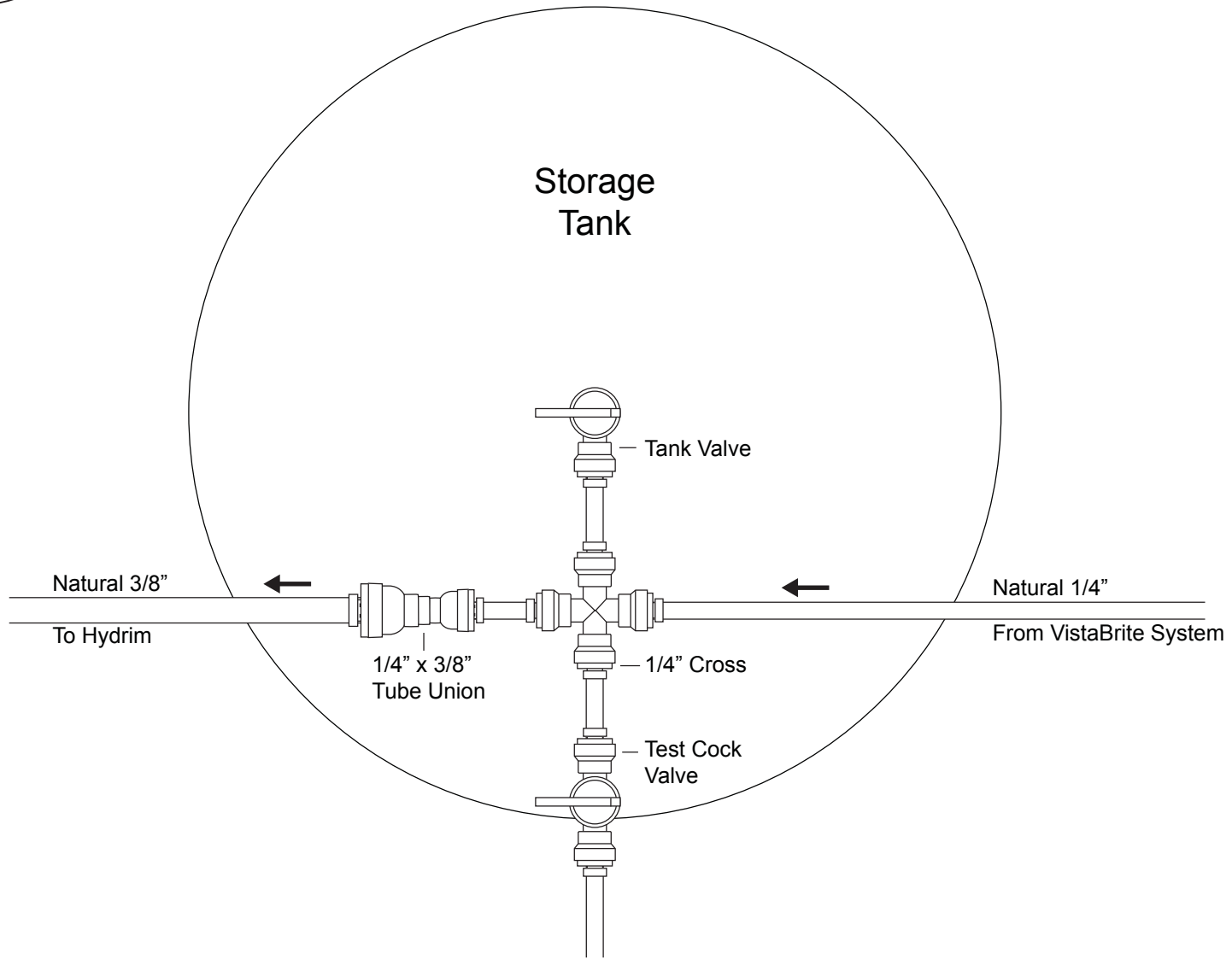
Storage Tank Tubing & Valve Assembly
